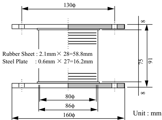
Outline of the laminated natural rubber bearing
